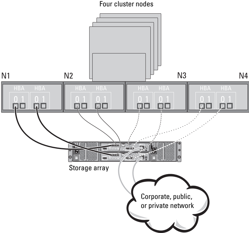
Figure 2-9. Four Cluster Nodes Connected to Two Controllers
