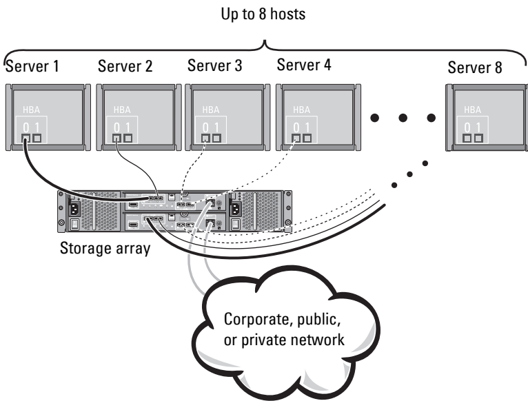
Figure 2-7. Eight Hosts Connected to Two Controllers
