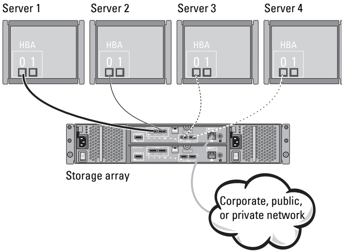
Figure 2-3. Four Hosts Connected to a Single Controller
