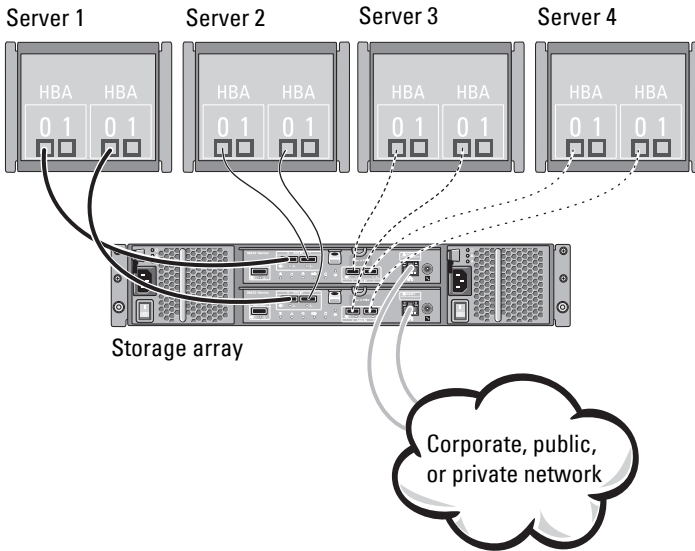
Figure 2-5. Four Hosts Connected to Two Controllers
