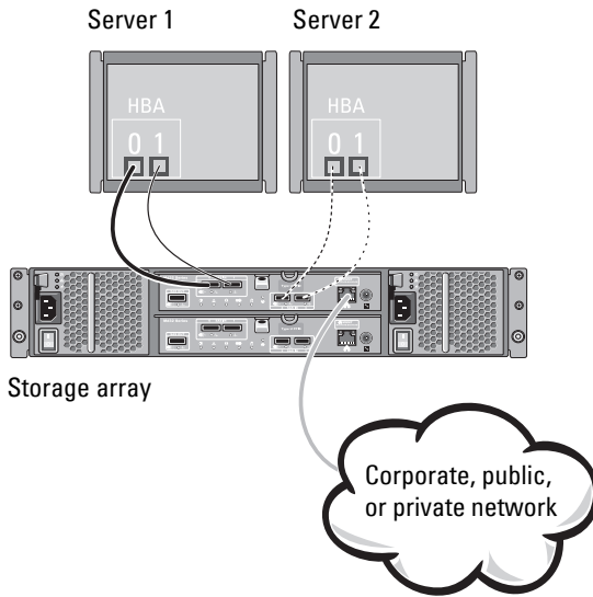
Figure 2-2. Two Hosts Connected to a Single Controller
