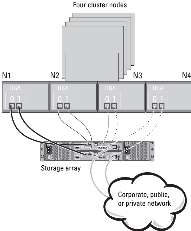
Figure 2-8. Four Cluster Nodes Connected to Two Controllers
