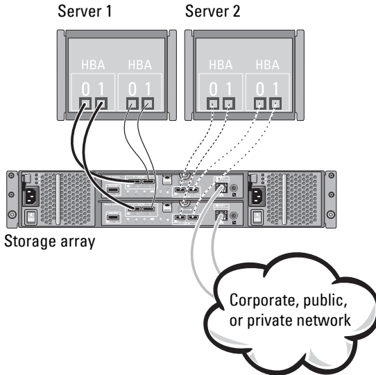
Figure 2-4. Two Hosts Connected to Two Controllers
