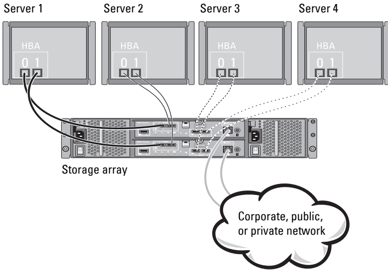
Figure 2-6. Four Hosts Connected to Two Controllers
