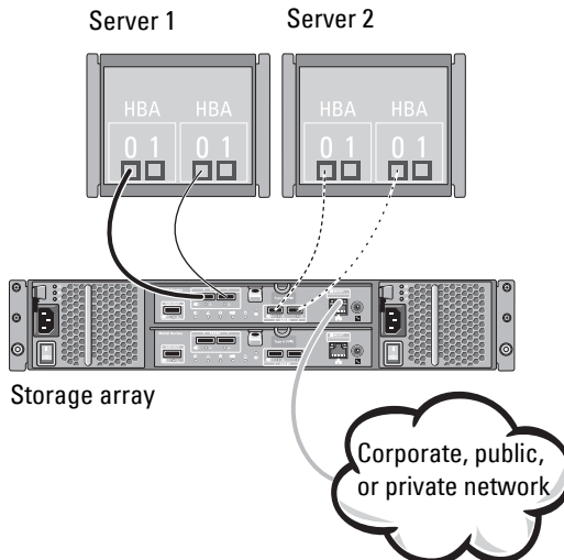
Figure 2-1. Two Hosts Connected to a Single Controller
